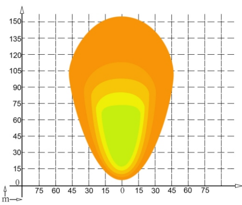
LOW BEAM PATTERN
