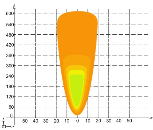
HIGH BEAM PATTERN
