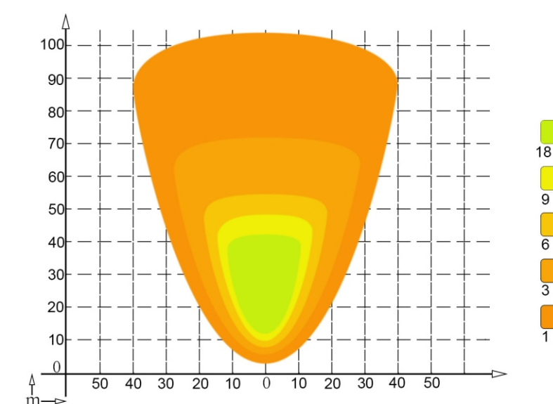
FLOOD BEAM
